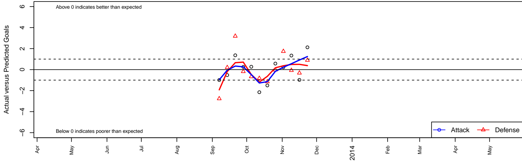
Desna SC B02 Dots are actual minus expected GF (blue circles) and GA (red triangles). Blue line is smoothed change in attack strength. Red is smoothed change in defense strength.
